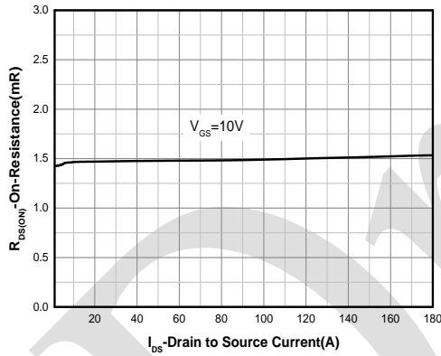
On-Resistance vs. Drain Current (4)
