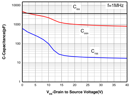
Capacitance
