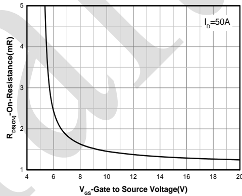
On-Resistance vs. Gate-to-Source Voltage (4)
